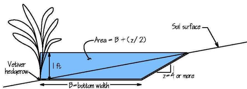
Figure 11. A trapezoid can be used to approximate the cross-sectional area of water contained by vetiver where a level section is used to increase the flow area behind the vetiver.
