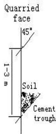
Fig. 1 Sketch of cement trough established on the quarried face
